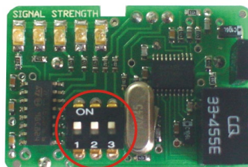
3-way Dipswitch
